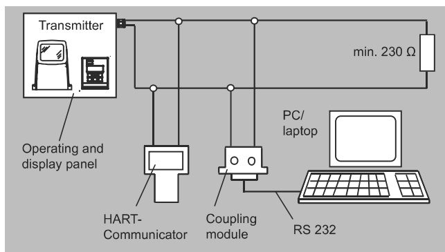
HART communication
